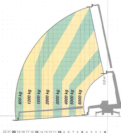
ROTO 60.24 MCSS FORKS ON STABILIZERS THROUGH 360°
