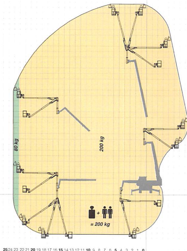
ROTO 60.24 MCSS SPACE SYSTEM THROUGH 360°
